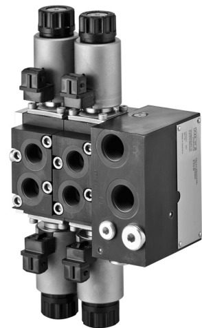
Proportional directional spool valve Type EDL
