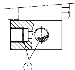
1 Screen filters and filter elements
